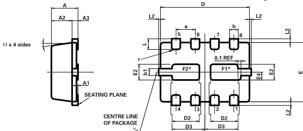
MLP832 PACKAGE OUTLINE (3mm x 2mm Micro Ledged Package)
